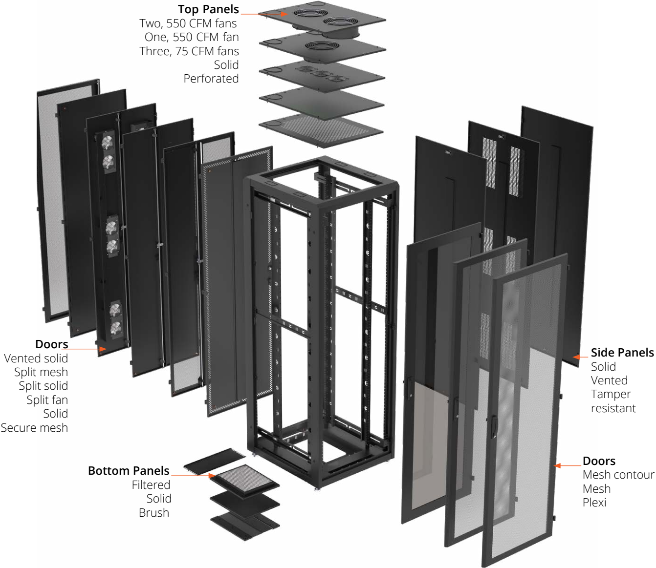
84"H x 29"W x 32"D frame shown, four top cabinet knockouts are part of 29" frames only, not all accessories shown are compatible with smaller cabinets
