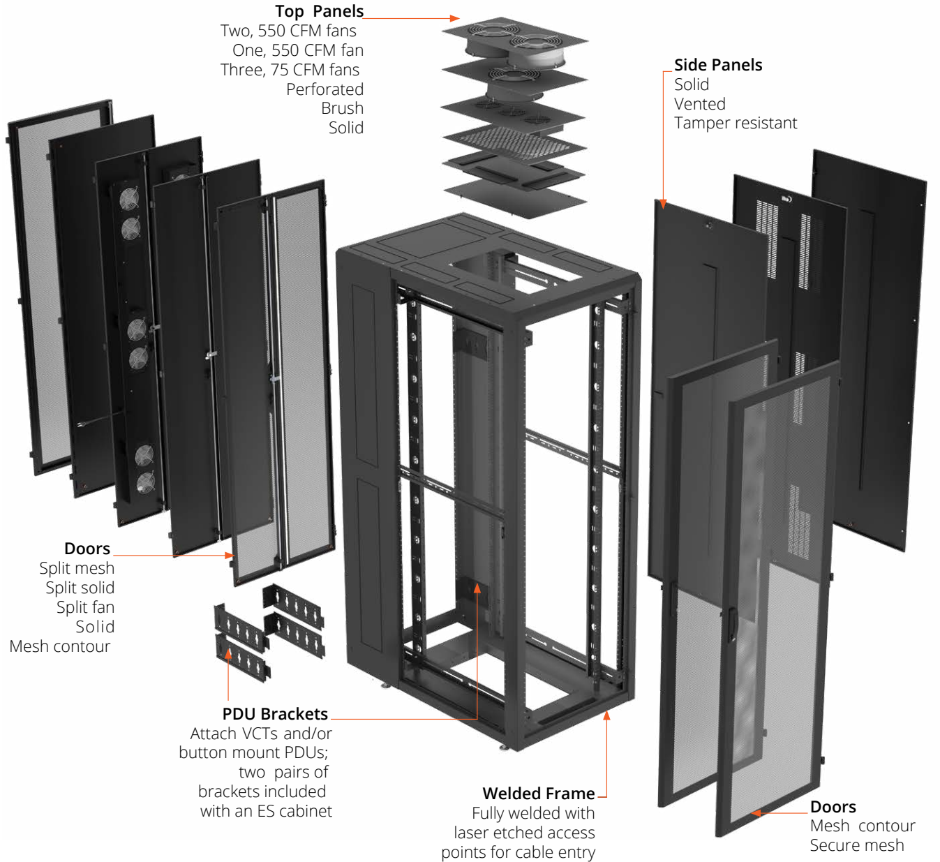
84"H x 30"W x 48"D frame shown, six top cabinet knockouts are part of 30/32" frames only
